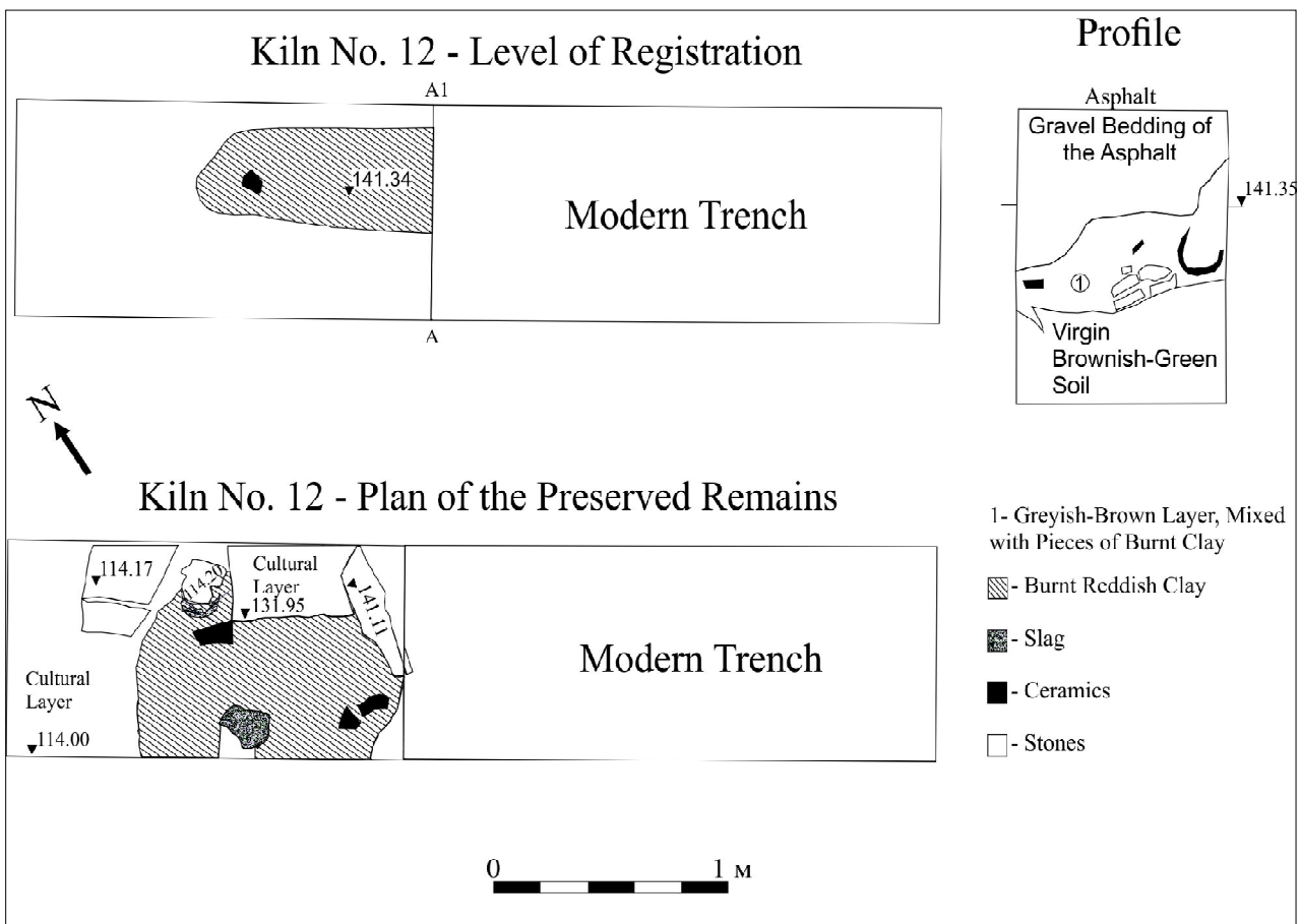
Figure 29 – Kiln No. 12 – plan and profile (K. Chakarov)
